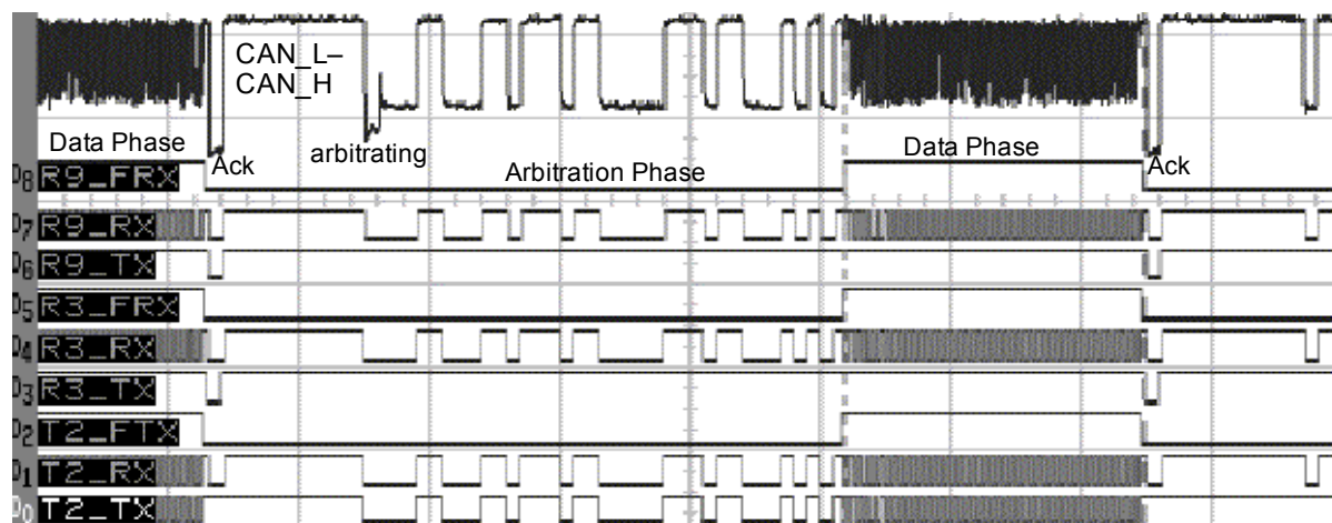
Figure 12 CAN FD Frame with 64 Data Bytes and 12 MBit/s in the Data-Phase
