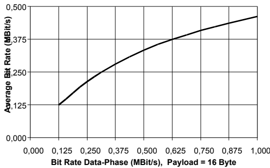
Figure 8 CAN FD Example for long Bus Lines
