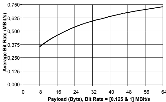
Figure 9 Average Bit Rates for long Bus Lines
