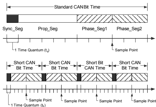
Figure 5 Standard and Short CAN Bit Time
