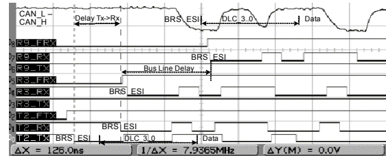
Figure 11 CAN FD Transceiver Loop Delay
