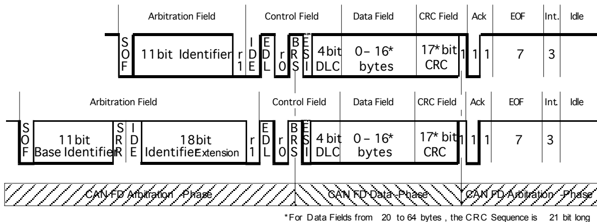
Figure 4 CAN FD Data Frame Format with 11 bit identifier and with 29 bit identifier
